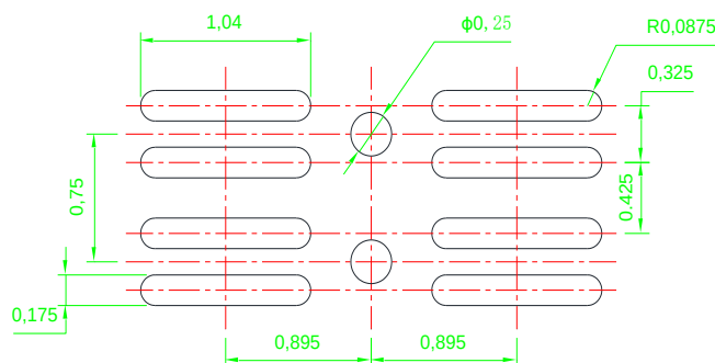
Land Pattern(Reference)
